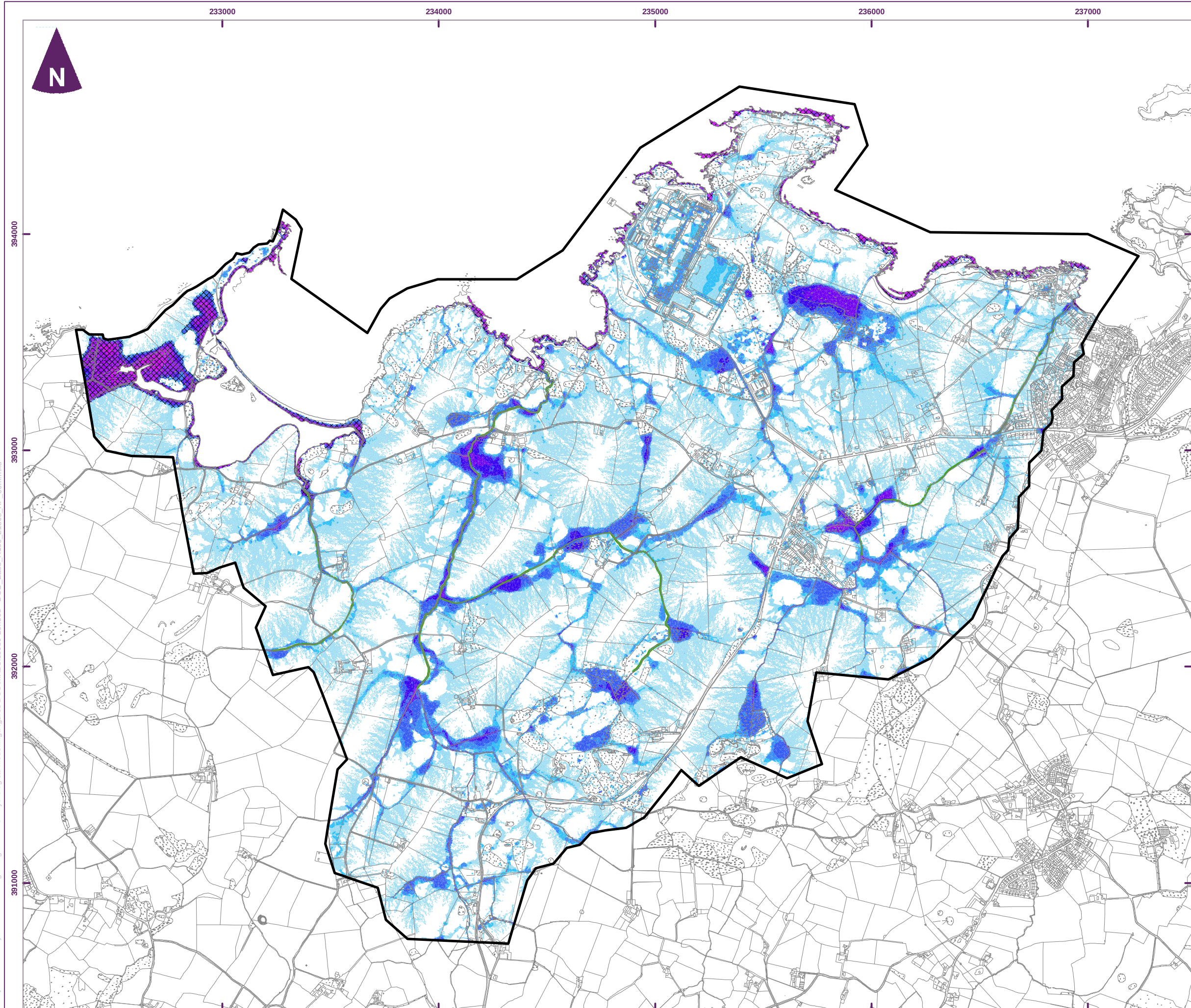
Figure 39 DCO baseline peak pluvial depth 1:100 year AEP 60 min duration climate change 2180s - reasonably foreseeable
